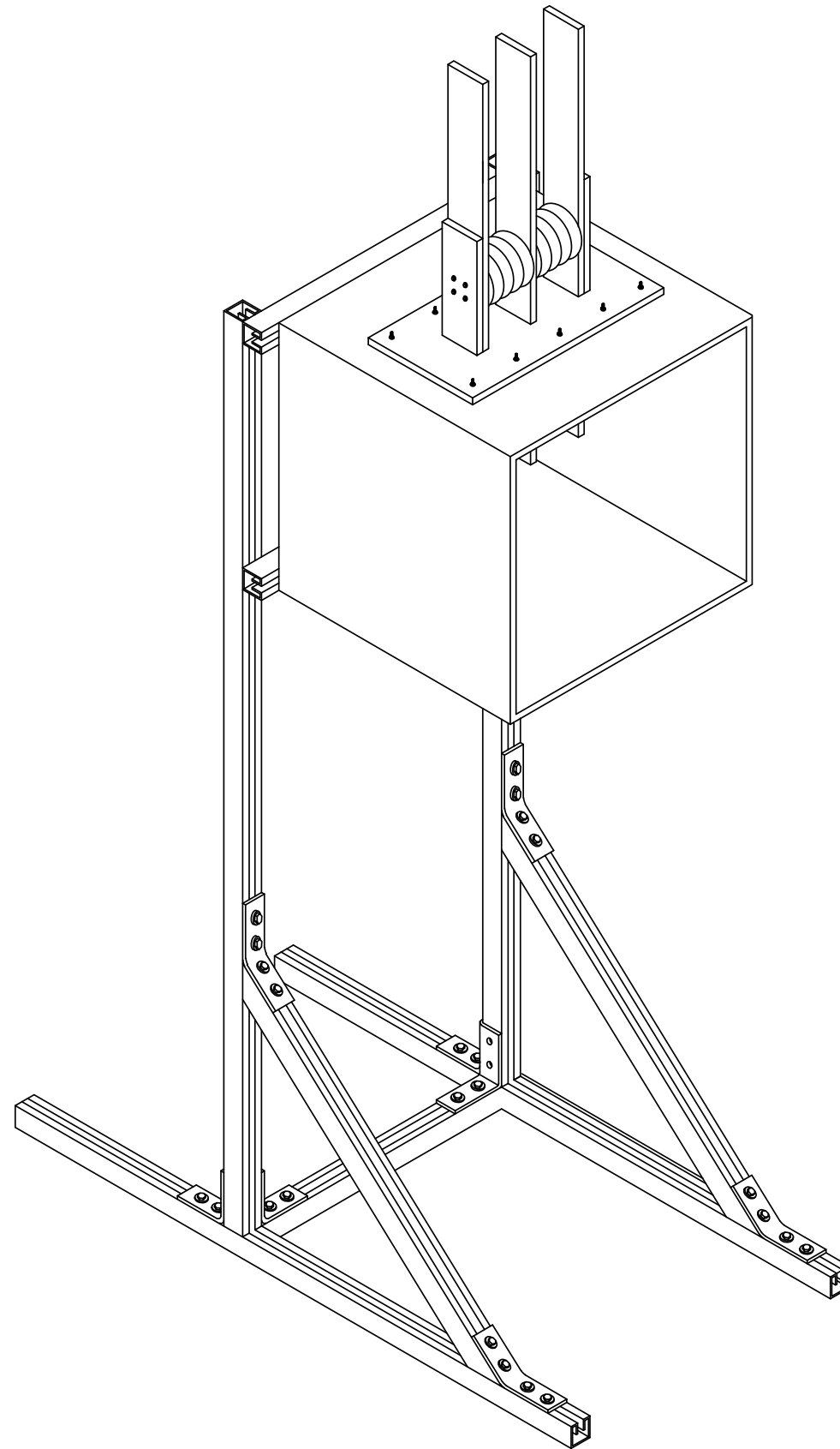
ALUMINUM AND COPPER BUS BARS INSERT
